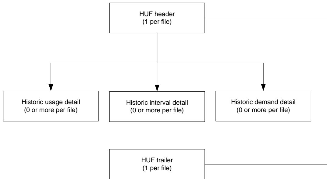
Figure 2. HUF Structure
